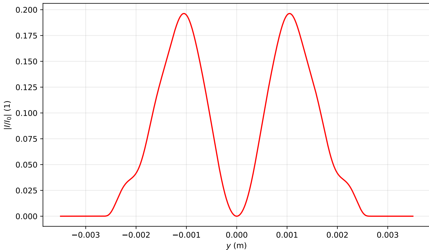
Intensity profile I(x=0, y, z=3.981)/I_0 , \text{Pin}=1.0\text{Pcr} , artificial time
